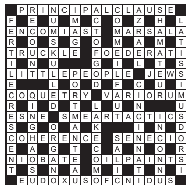
Solution Polymath 1,134
